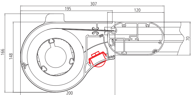
Cross sections and dimensions Sottezza II LED
